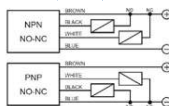
4 wires (NO+NC)
